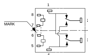
TERMINAL ARRANGEMENT/ INTERNAL CONNECTIONS (BOTTOM VIEW)
