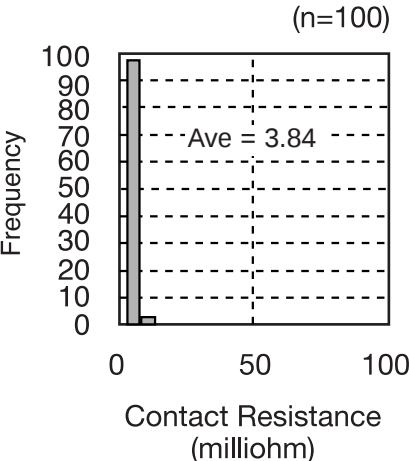
N.O. contact - Distribution of contact resistance
