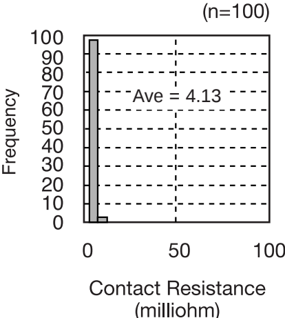
N.C. contact - Distribution of contact resistance
