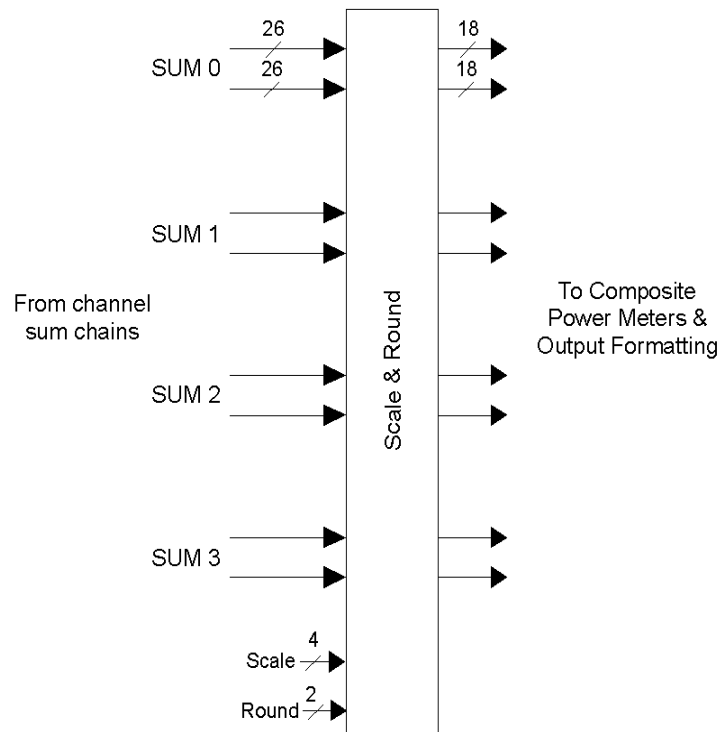
Figure 35. Final Sum Chain Scale and Round Block
