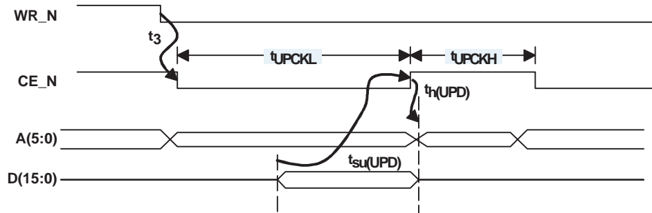
Figure 40. Write Diagrams
