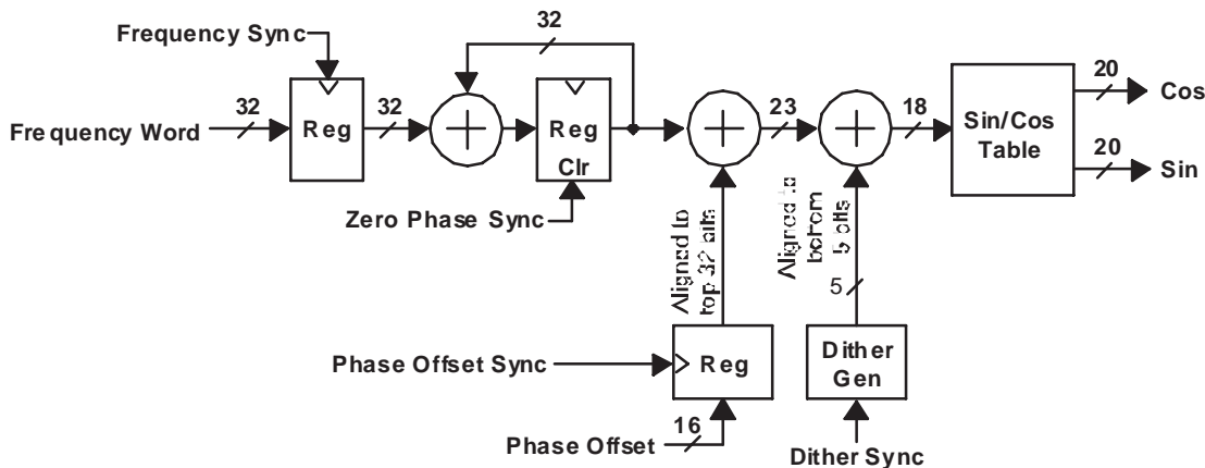
Figure 31. Transmit NCO
