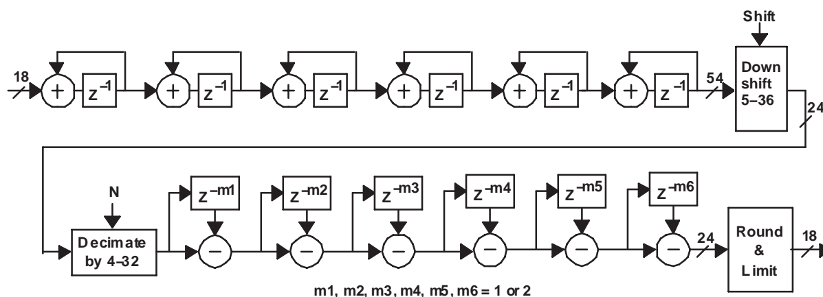
Figure 13. Six Stage CIC Filter
