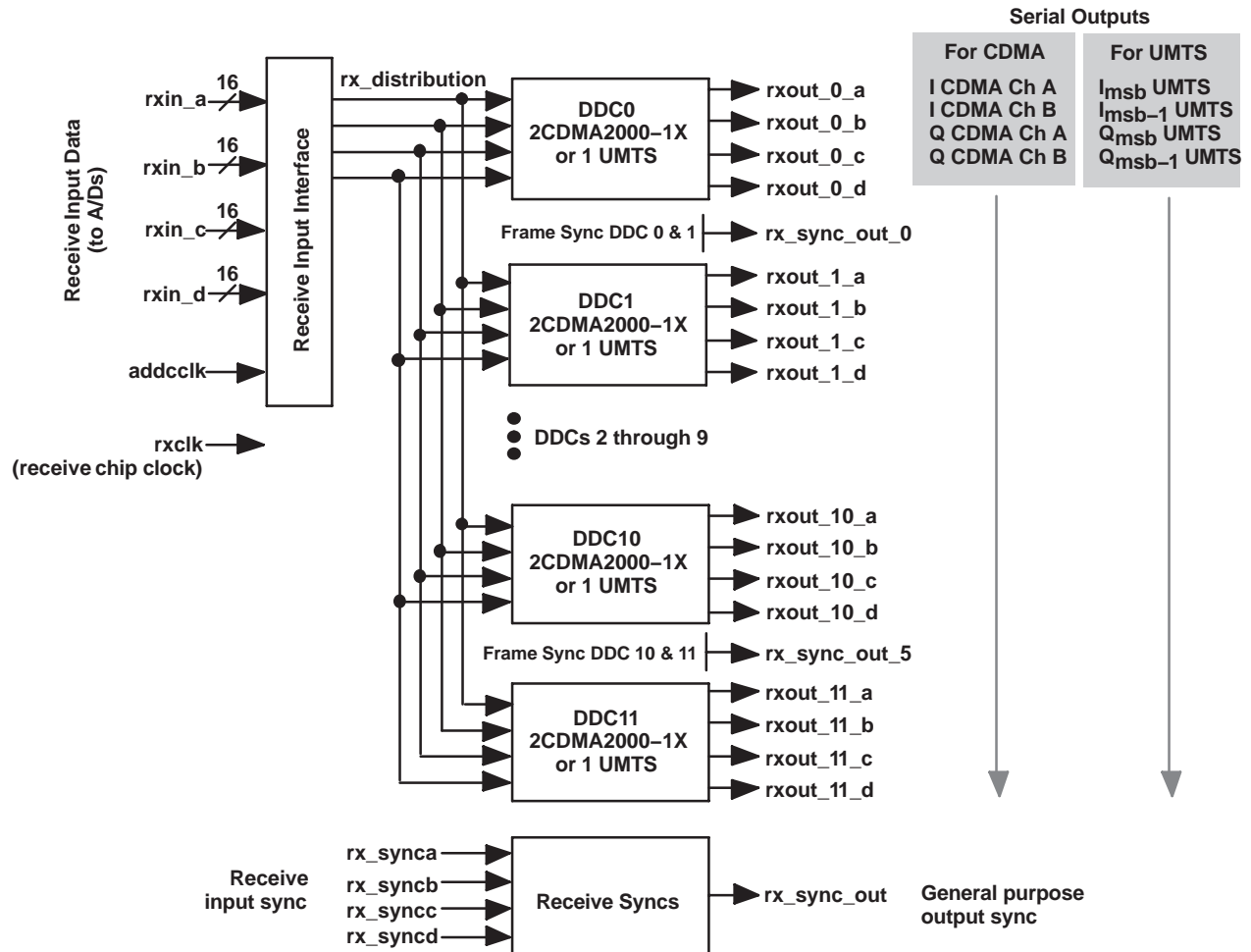
Figure 1. Receive Section
