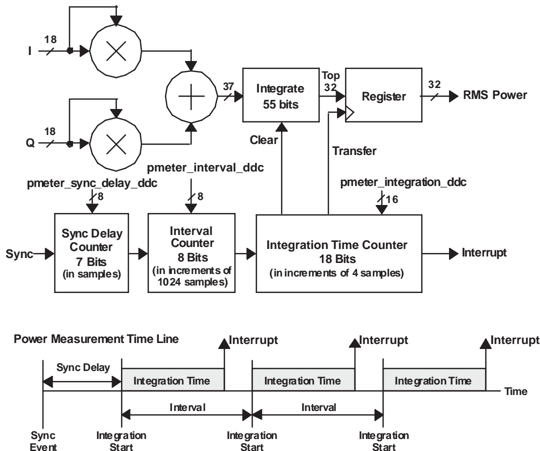
Figure 15. Receive Power Meter and Timing
