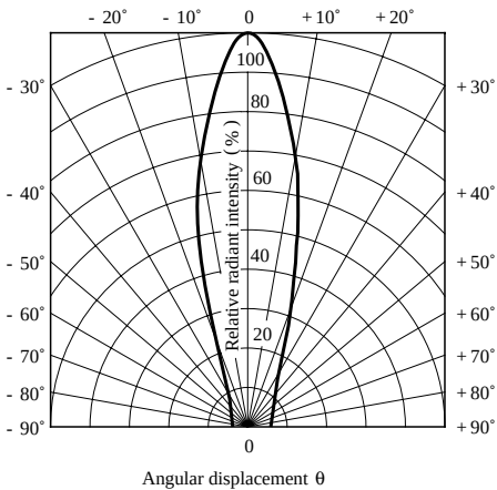
Fig. 9 Radiation Diagram
