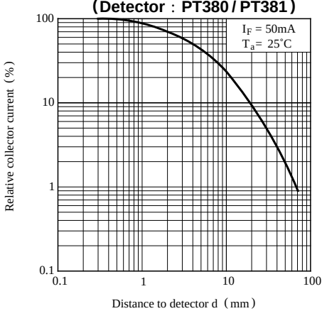
Fig. 8 Relative Collector Current vs. Distance
