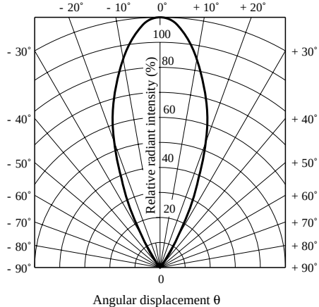
Fig. 11-a Radiation Diagram (GL560) ( T_a = 25^\circ\text{C} )
