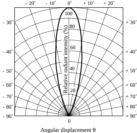
Fig. 11-b Radiation Diagram (GL561) ( T_a = 25^\circ\text{C} )
