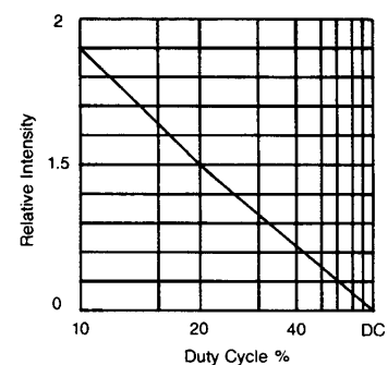
Fig. 6. Luminous Intensity vs. Duty Cycle %
