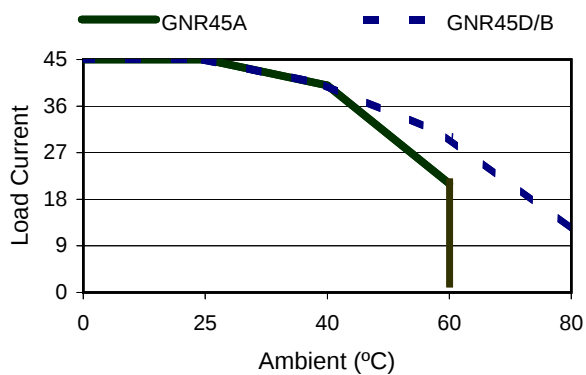
GNR45 Series Derate Curves
