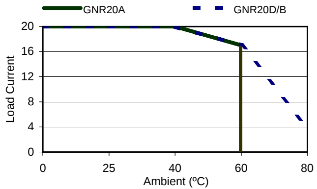
GNR20 Series Derate Curves
