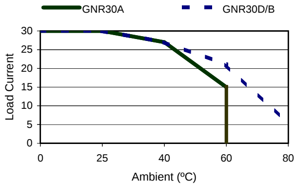
GNR30 Series Derate Curves
