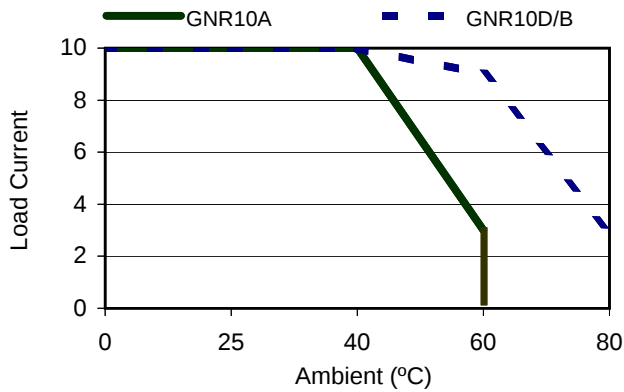
GNR10 Series Derate Curves
