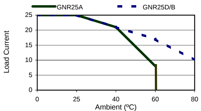
GNR25 Series Three-Phase Derate Curves (Ratings per Phase)
