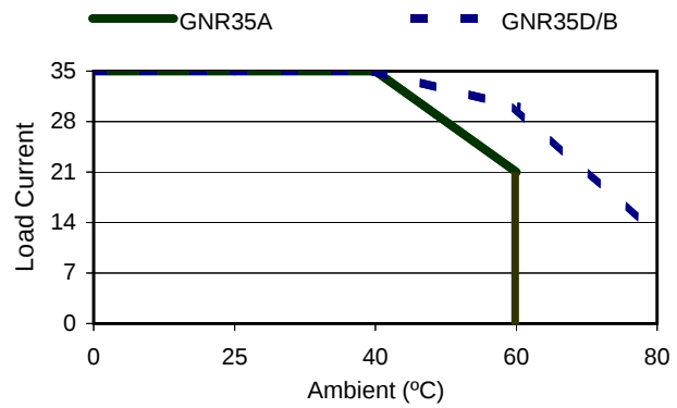
GNR35 Series Derate Curves
