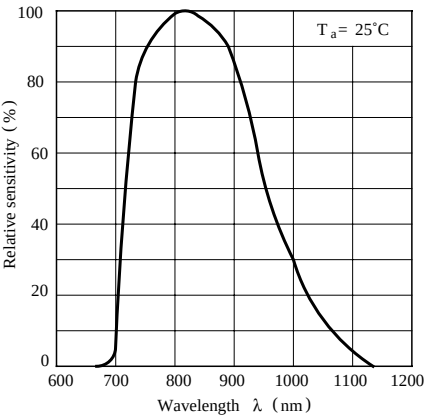
Fig.15 Spectral Sensitivity (Detecting Side)
