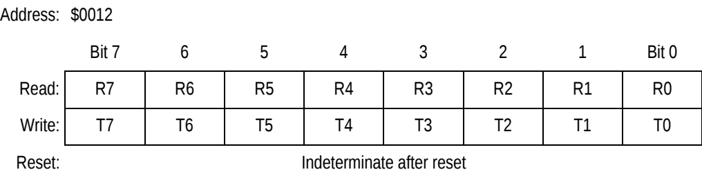
Figure 20-15. SPI Data Register (SPDR)
