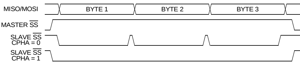
Figure 20-12CPHA/ \overline{SS} Timing
