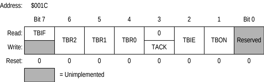
Figure 21-2. Timebase Control Register (TBCR)
