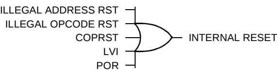
Figure 19-6. Sources of Internal Reset
