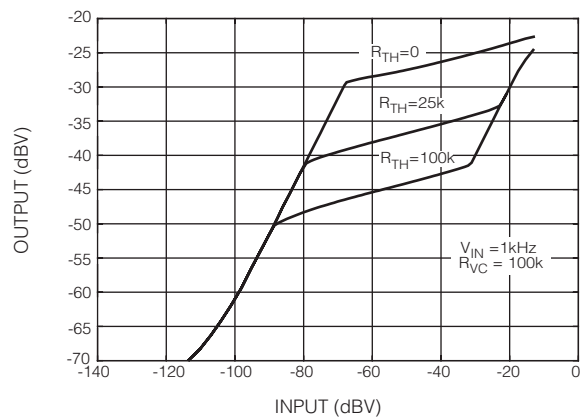
Fig. 6 Input vs Output Threshold Settings
