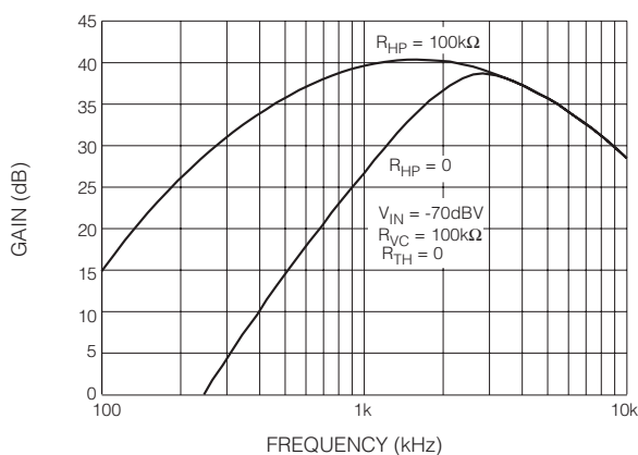
Fig. 8 Frequency Response vs R_{HP}
