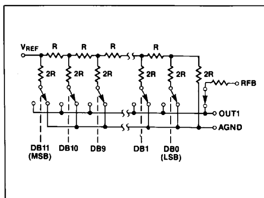
Figure 1. Simplified D/A Circuit of MX7545
