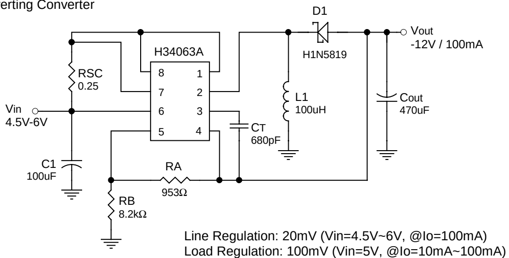
Fig.6 Voltage Inverting Converter
