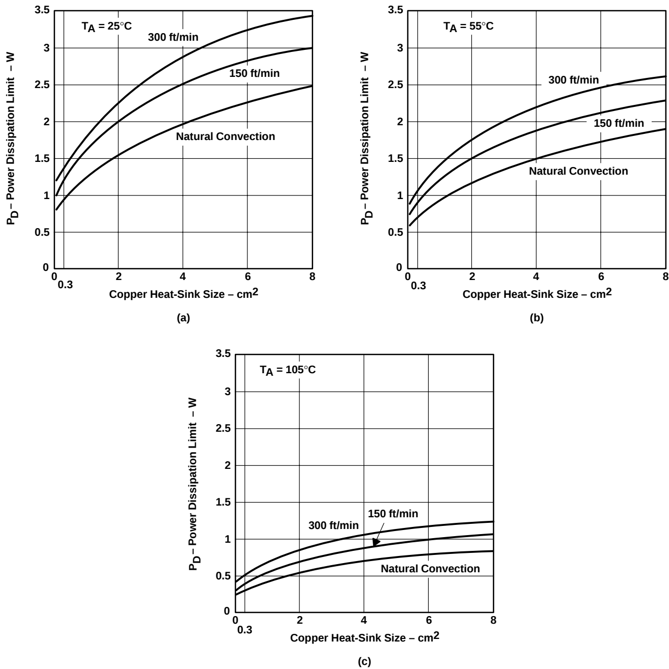
Figure 48. Power Ratings of the PWP Package at Ambient Temperatures of 25°C, 55°C, and 105°C
