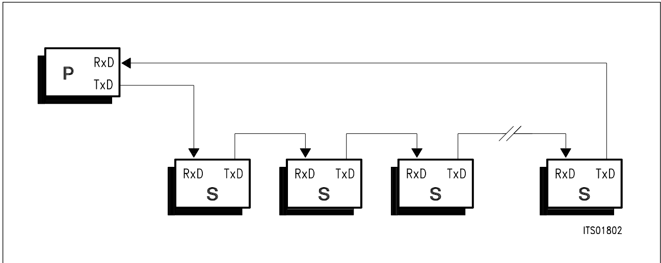
Figure 30 SDLC Loop
