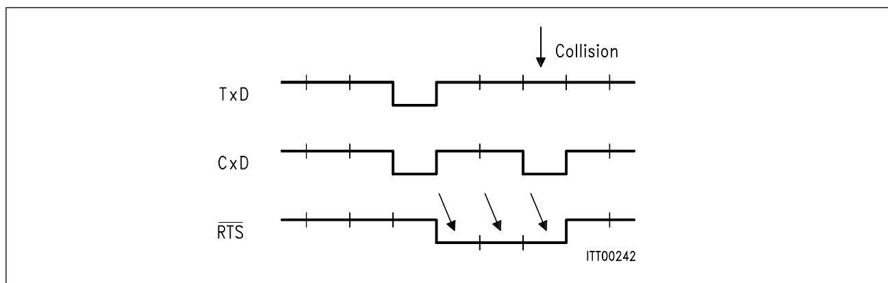
Figure 41 Request-to-Send in Bus Operation
