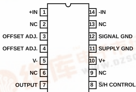
HA-5330 (PDIP, Cerdip) TOP VIEW
