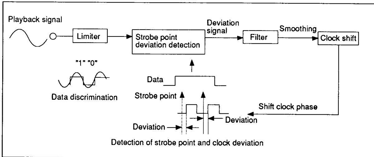
Figure 6 ASPC Structure
