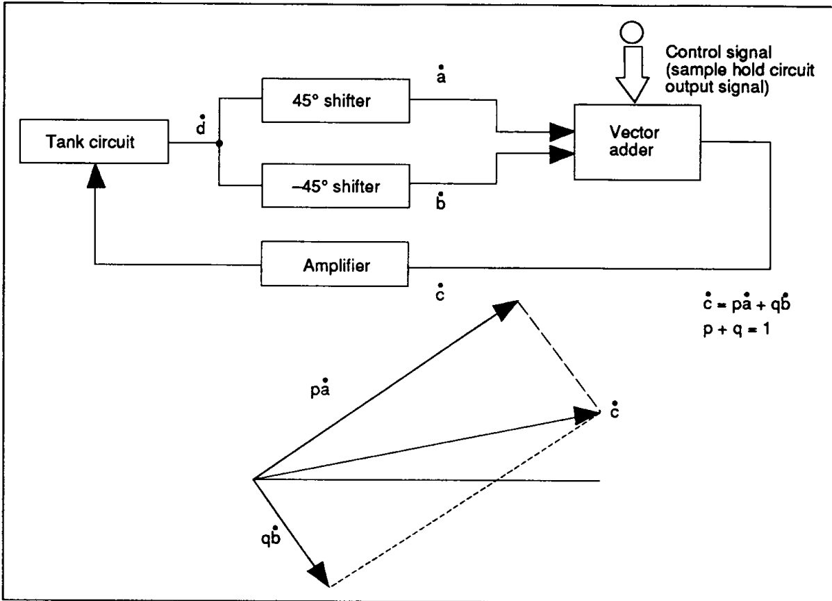
Figure 5 VCO Structure
