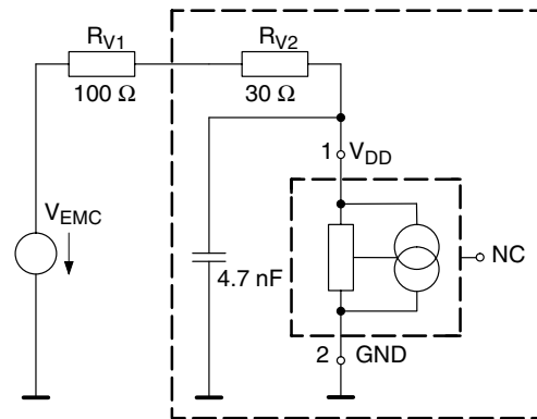
Fig. 5–3: Recommended EMC test circuit
