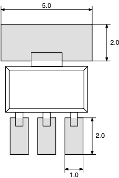
Fig. 3–3: Recommended pad size SOT-89B Dimensions in mm
