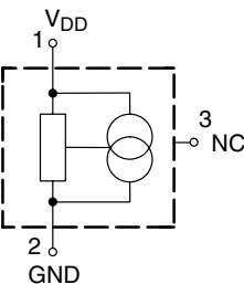
Fig. 1–1: Pin configuration
