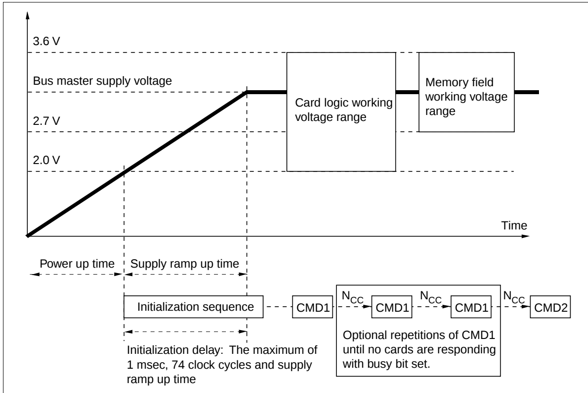
Power-up Diagram
