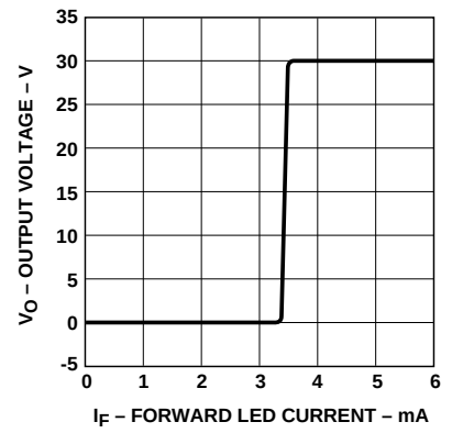
Figure 15. Transfer Characteristics.
