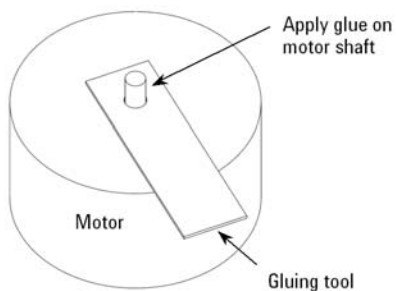
Motor inserted with gluing tool
