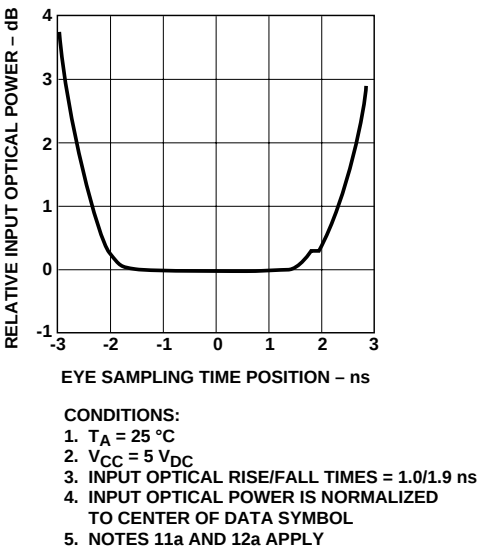
Figure 9. HFBR-5301, Relative Input Optical Power vs. Eye Sampling Time Position.
