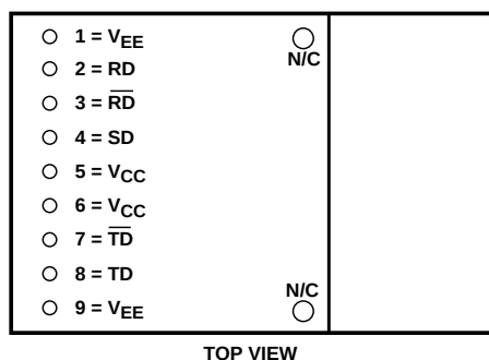
Figure 3. Pinout Diagram.
