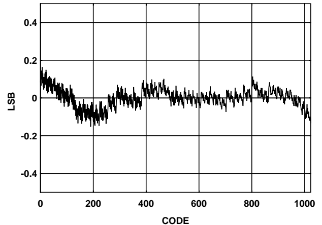
FIGURE 18. INTEGRAL NONLINEARITY
