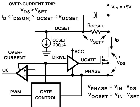
FIGURE 6. OVER-CURRENT DETECTION
