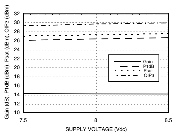
Gain, Power & OIP3 vs. Supply Voltage @ 10 GHz, Fixed Vgg1
