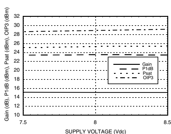
Gain, Power & OIP3 vs. Supply Voltage @ 10 GHz, Idd= 160mA
