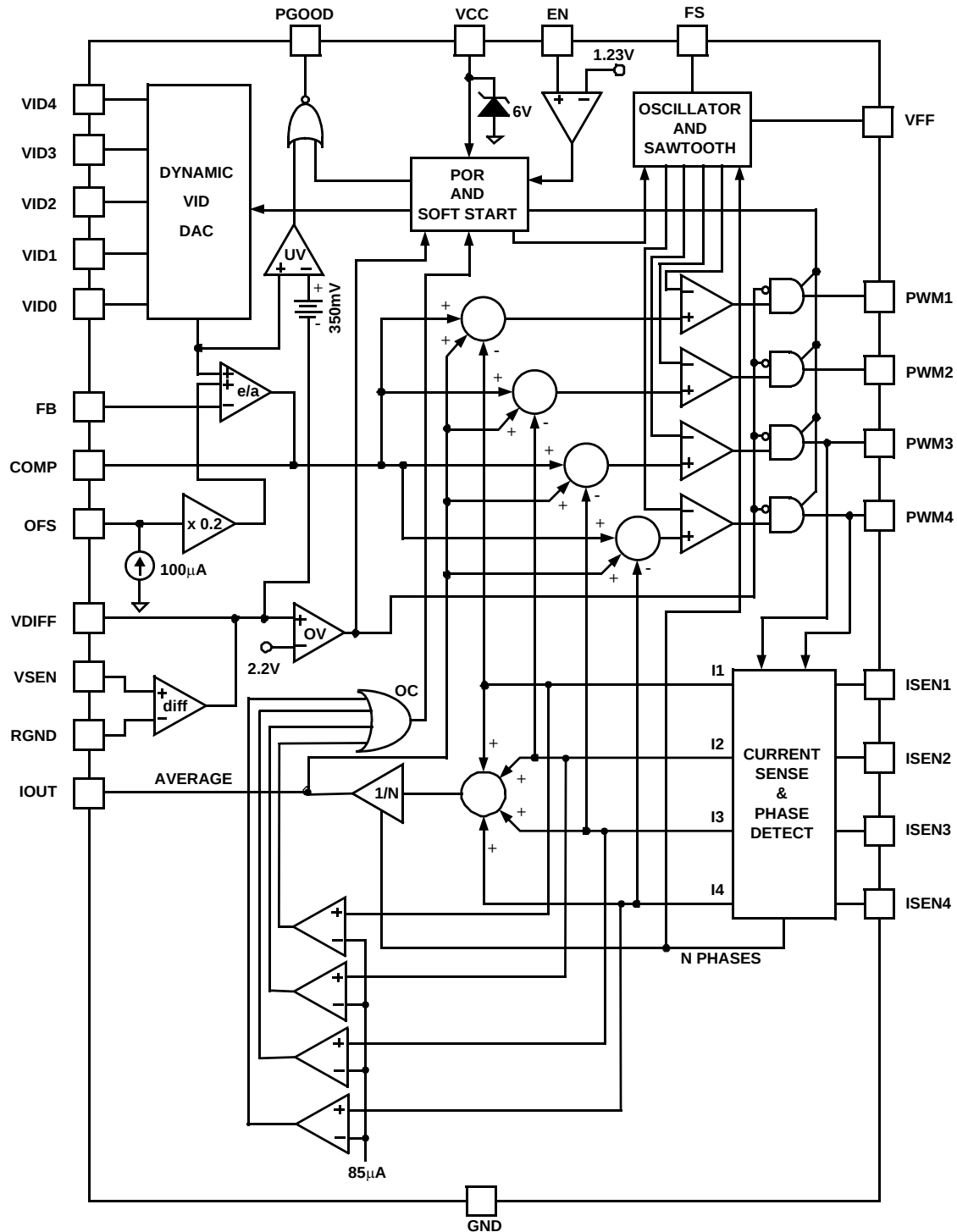
FIGURE 12. BLOCK DIAGRAM
