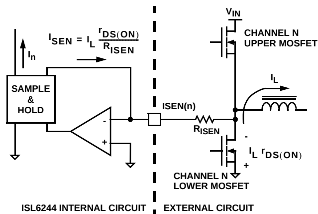
FIGURE 15. INTERNAL AND EXTERNAL CURRENT-SENSING CIRCUITRY
