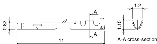
Female contact
