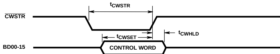
FIGURE 4. CONTROL WORD TIMING
