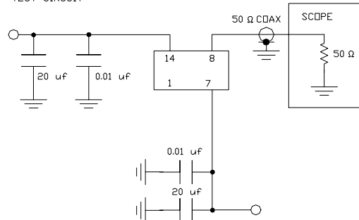
TEST CIRCUIT
