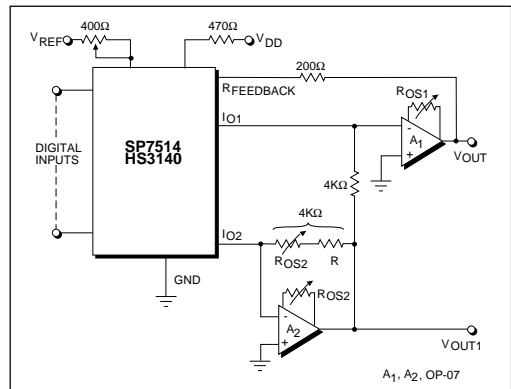
Figure 3. Bipolar Operation
