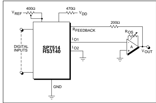
Figure 2. Unipolar Operation
