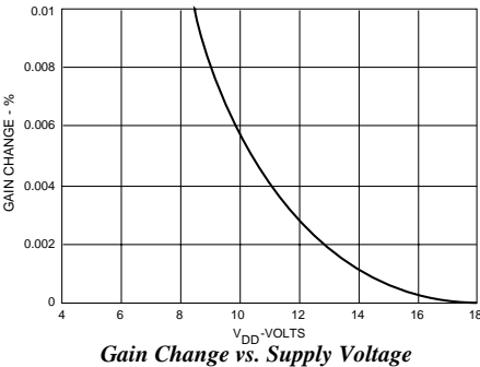
Gain Change vs. Supply Voltage
