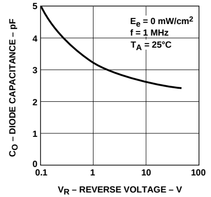
Figure 16. Diode Capacitance vs. Reverse Voltage.
