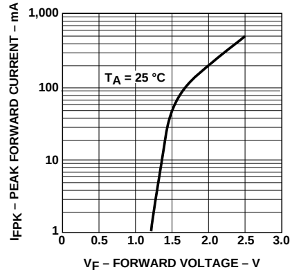
Figure 2. Peak Forward Current vs. Forward Voltage.
