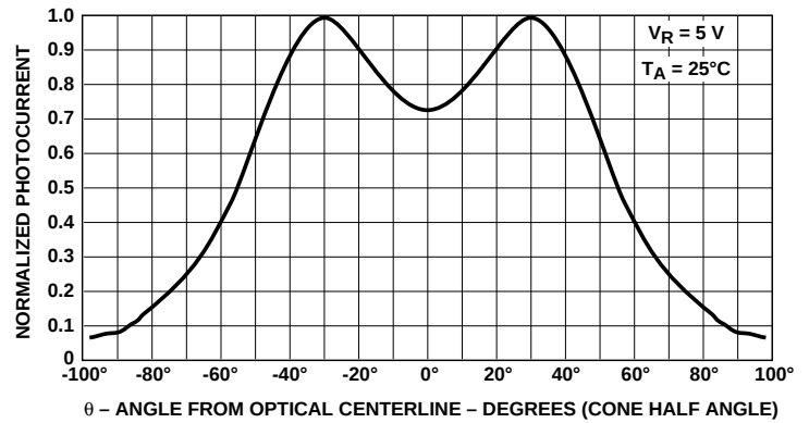
Figure 18. Relative Radiant Intensity vs. Angular Displacement. HSDL-5400.
