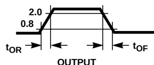
FIGURE 11. RISE AND FALL TIMES
