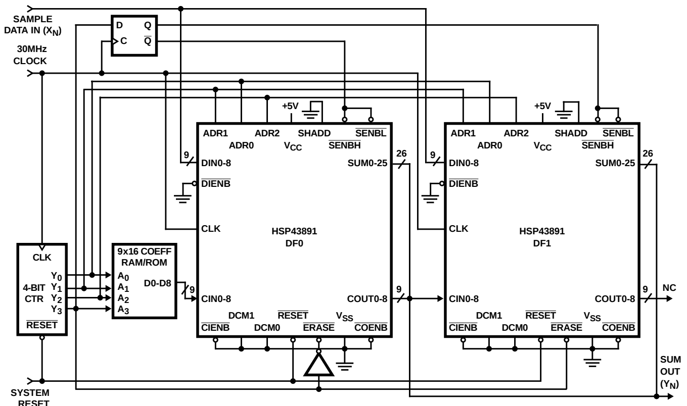
FIGURE 5. HSP43891 30MHz, 16-TAP FIR FILTER CASCADE APPLICATION SCHEMATIC
