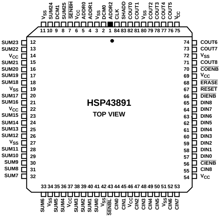
84 LEAD PLASTIC LEADED CHIP CARRIER (PLCC)
