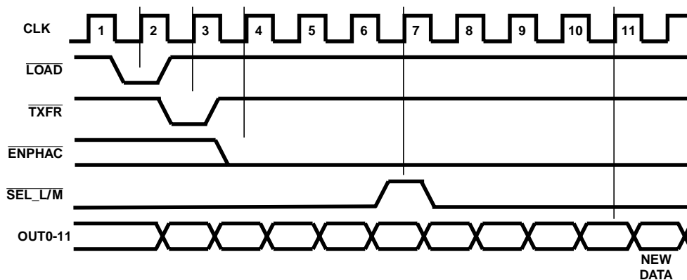
FIGURE 3. I/O TIMING
