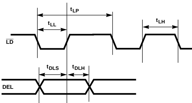
FIGURE 5. ASYNCHRONOUS TIMING
