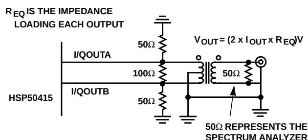
FIGURE 19. DAC OUTPUTS
