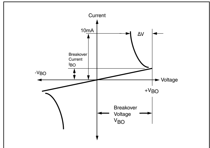
Figure 8.7 V-I Characteristics
