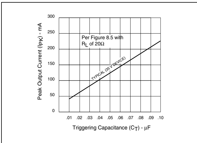
Figure 8.6 Peak Output Current vs Triggerring Capacitance
