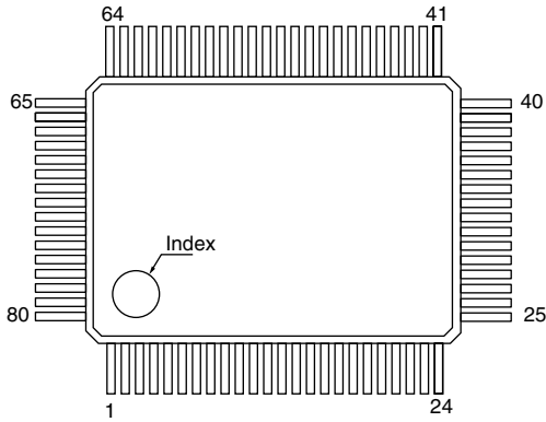
top view 80-pin Gullwing Package
