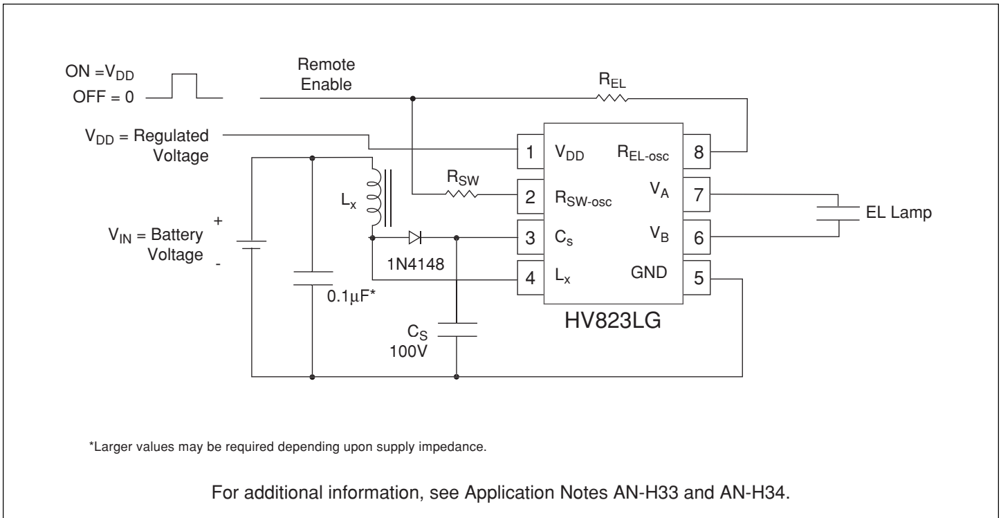
Figure 5: Split Supply Configuration
