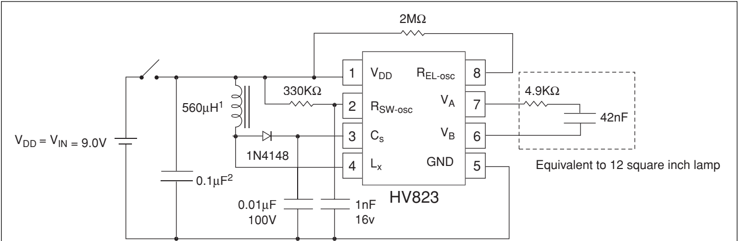
Figure 3: Typical 9.0V Application*
