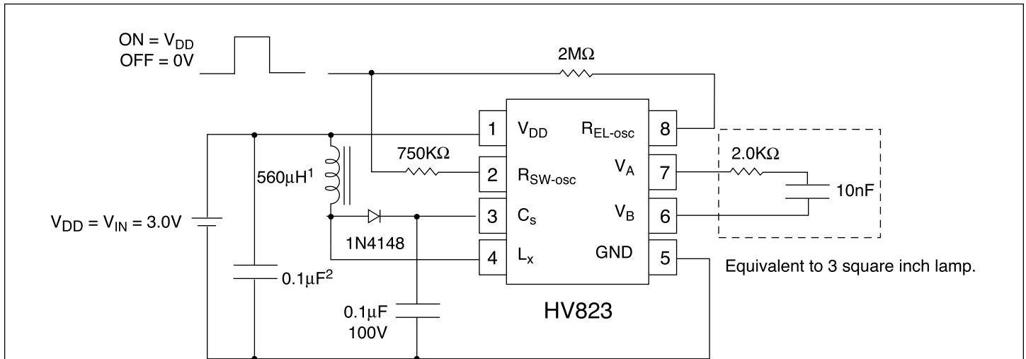
Figure 1: Test Circuit, V_{IN} = 3.0V (Low input current with moderate output brightness).
