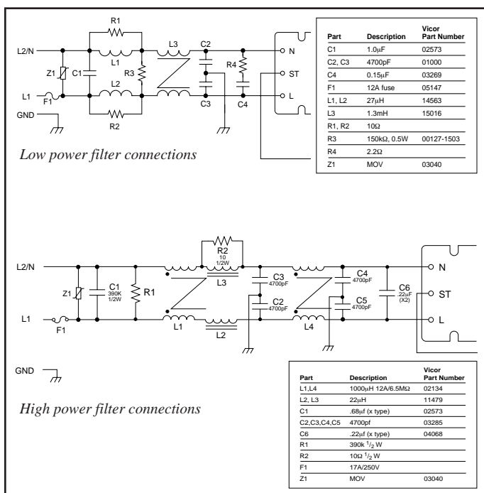
Figure 11—Filter connections
