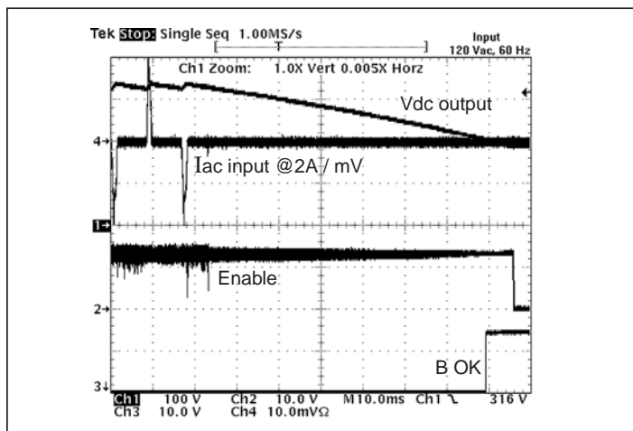
Figure 3—Power down, from 120Vac
