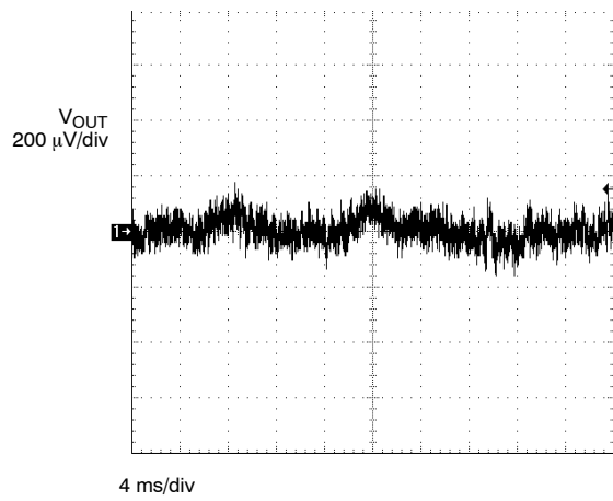
Output Noise
