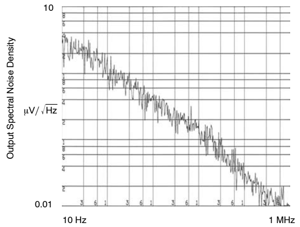
Noise Spectrum
