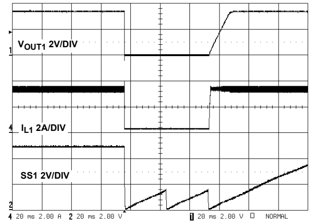
FIGURE 10. OVERCURRENT HICUP MODE OPERATION
