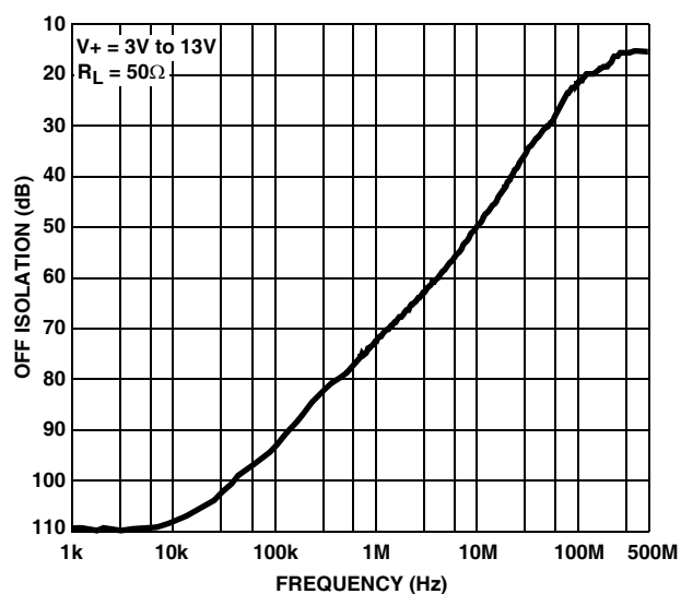
FIGURE 16. OFF ISOLATION
