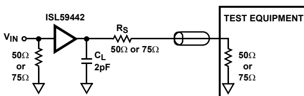
FIGURE 21C. BACKLOADED TEST CIRCUIT FOR VIDEO CABLE APPLICATION. BANDWIDTH AND LINEARITY FOR R_L LESS THAN 500Ω WILL BE DEGRADED
