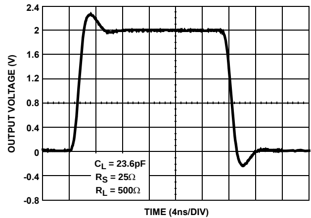
FIGURE 18. LARGE SIGNAL TRANSIENT RESPONSE
