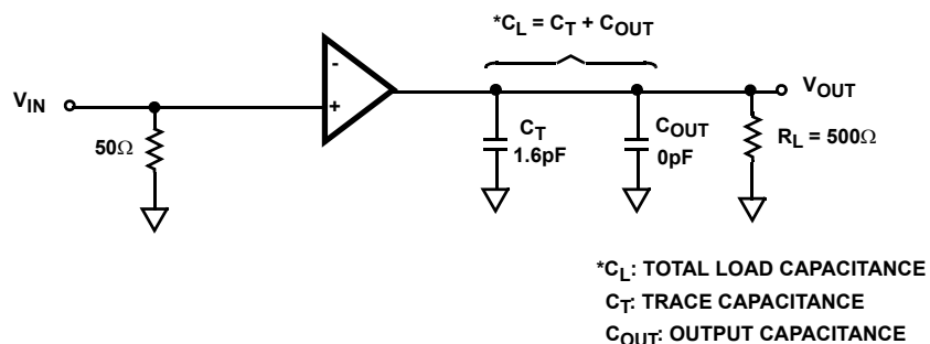
FIGURE 22A. SMALL SIGNAL 200mV p,p APPLICATION CIRCUIT
