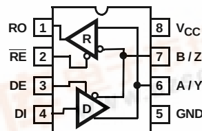
ISL81485 (SOIC, MSOP) TOP VIEW
