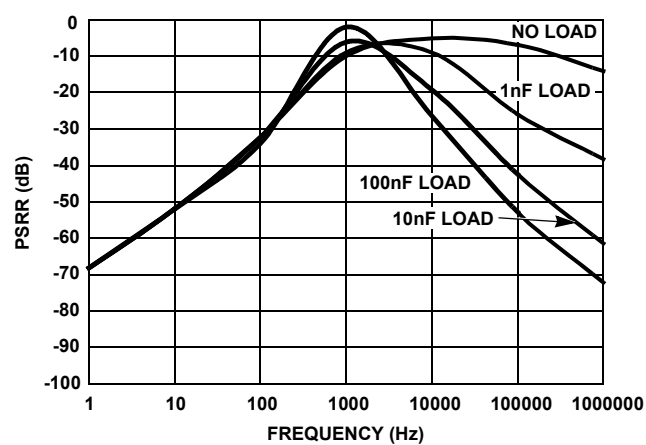
FIGURE 20. PSRR vs f vs C_L
