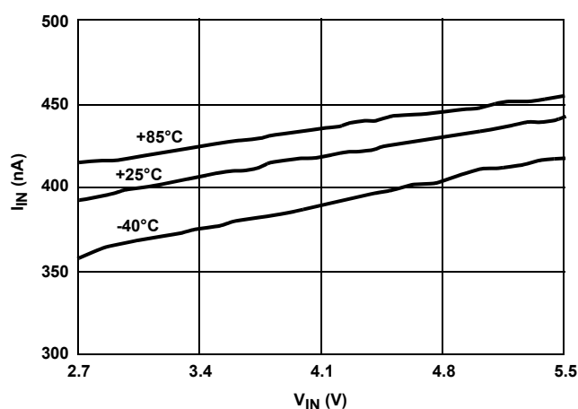
FIGURE 14. I_{IN} vs V_{IN} - 3 TEMPS
