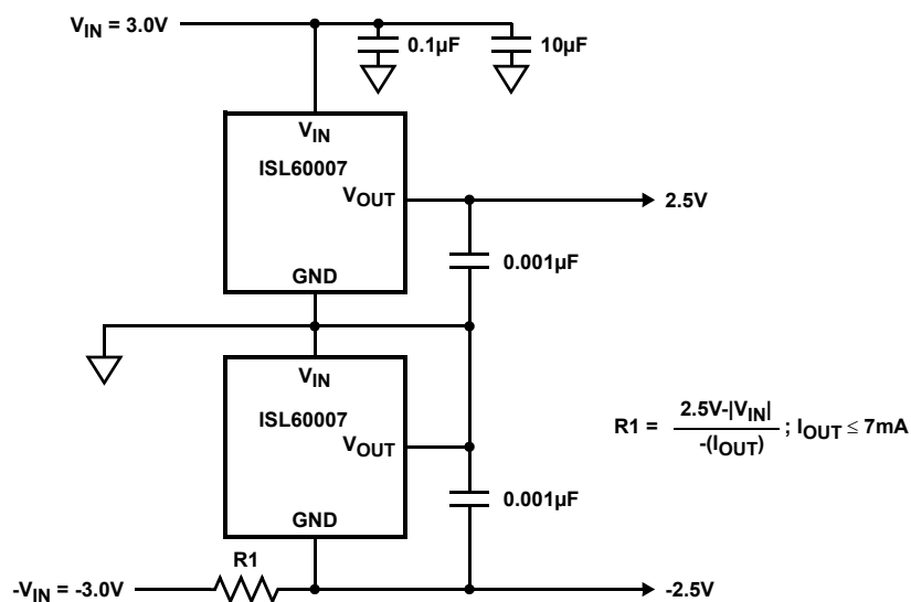
FIGURE 32. ±2.5V DUAL OUTPUT, HIGH ACCURACY REFERENCE
