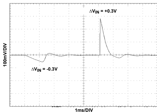
FIGURE 19. LINE TRANSIENT RESPONSE, C_L = 1nF
