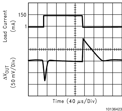
Load Transient Response ( V_{IN} = 3.2V )
