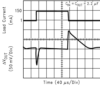
Load Transient Response ( V_{IN} = 3.2\text{V} )
