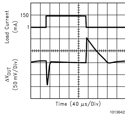
Load Transient Response ( V_{IN} = 4.2V )
