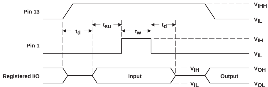
Figure 1. Preload Waveforms
