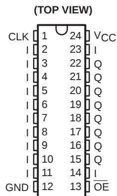
TIBPAL20R8' C SUFFIX . . . JT OR NT PACKAGE M SUFFIX . . . JT OR W PACKAGE
