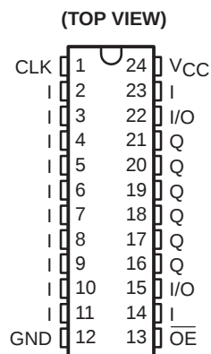
TIBPAL20R6' C SUFFIX . . . JT OR NT PACKAGE M SUFFIX . . . JT OR W PACKAGE
