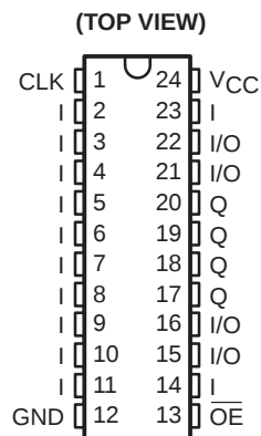
TIBPAL20R4' C SUFFIX . . . JT OR NT PACKAGE M SUFFIX . . . JT OR W PACKAGE
