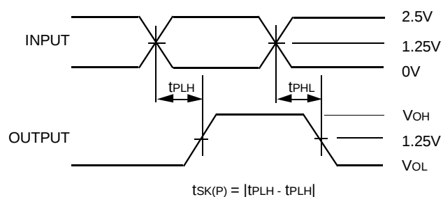
Pulse Skew
