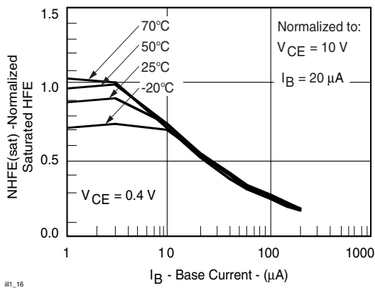
Figure 16. Normalized Saturated HFE vs. Base Current and Temperature
