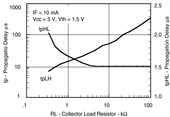
Figure 17. Propagation Delay vs. Collector Load Resistor
