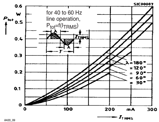
Fig. 9 Power Dissipation
