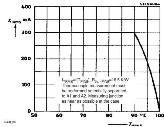
Fig. 6 Current Reduction
