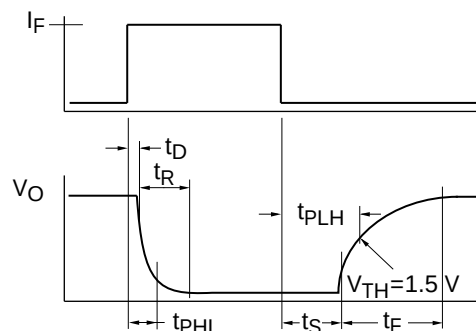
Figure 6. Switching timing
