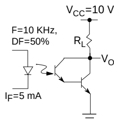
Figure 7. Switching schematic
